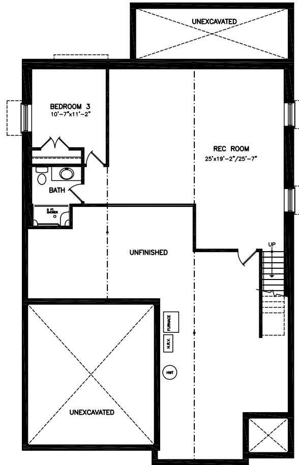
BASEMENT PLAN FINISHED AREA = 918 SQ.FT.
