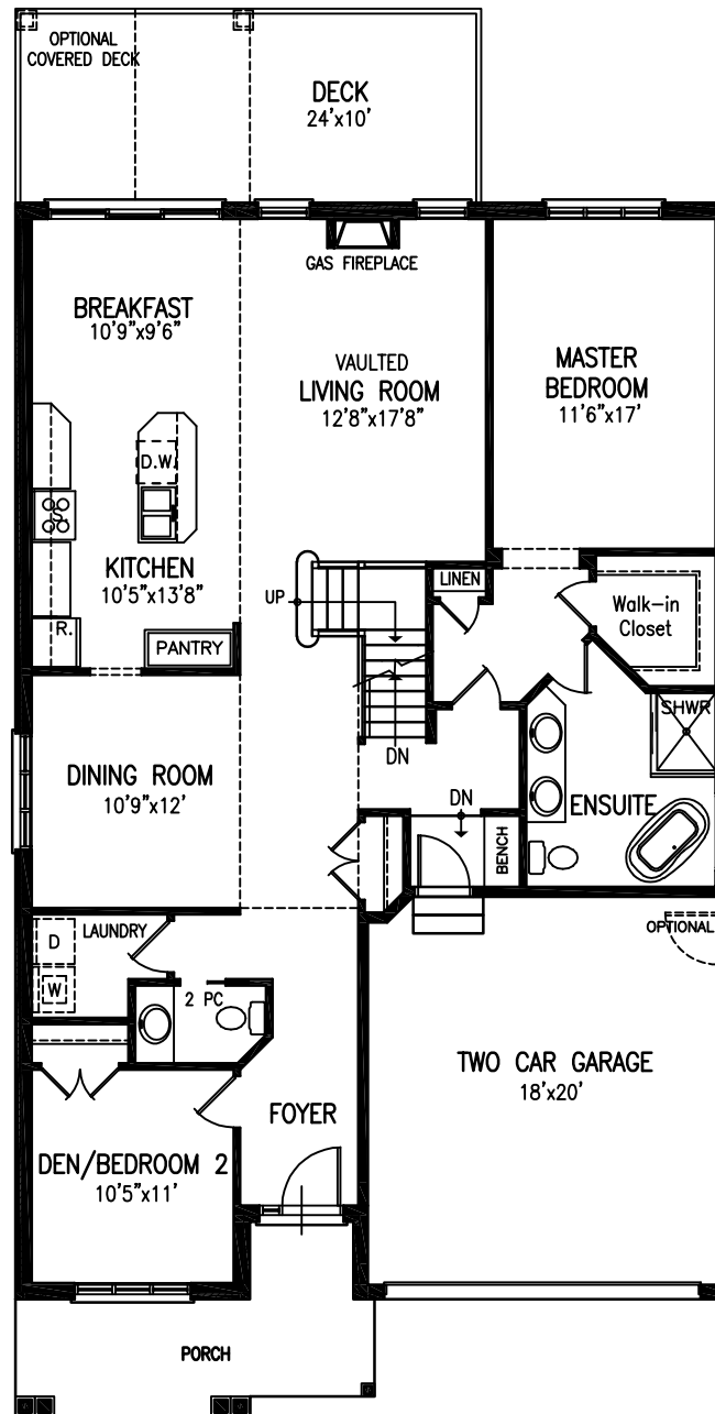
MAIN FLOOR PLAN - 1675 SQ.FT.
