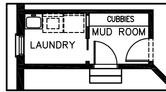
MAIN FLOOR LAUNDRY (WITH ALTERNATE SECOND FLOOR ONLY)
