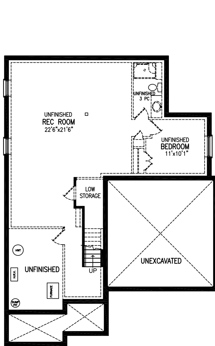
UNFINISHED BASEMENT PLAN OPTIONAL FINISHED AREA 1026 SQ.FT.
