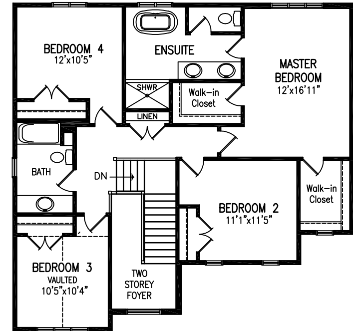
SECOND FLOOR PLAN - 1188 SQ.FT.
