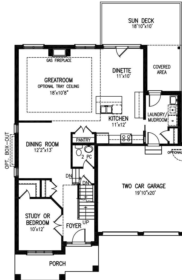
MAIN FLOOR PLAN - 1275 SQ.FT.
