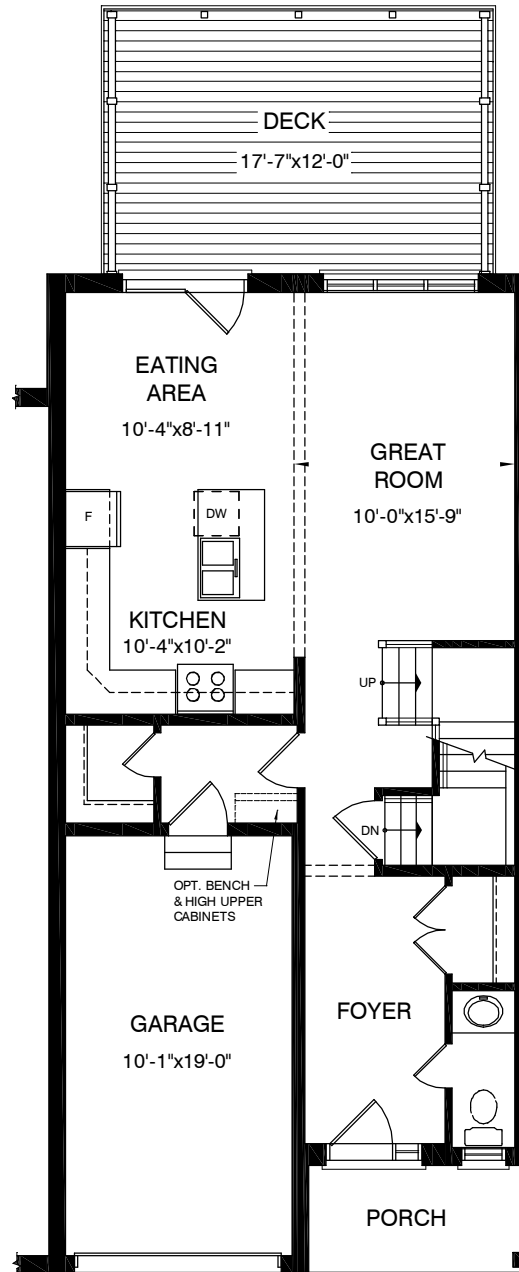
Main Floor
