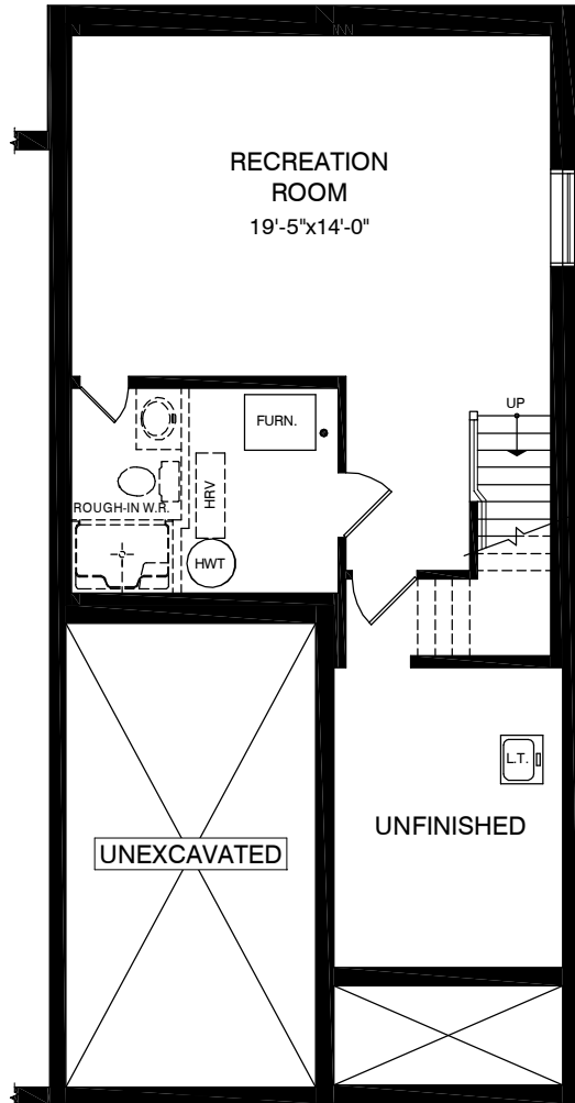
Basement Plan
