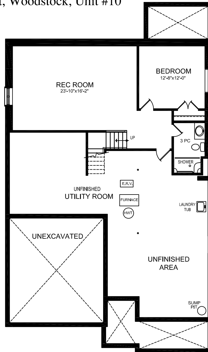
BASEMENT PLAN FINISHED AREA = 819 SQ.FT.
