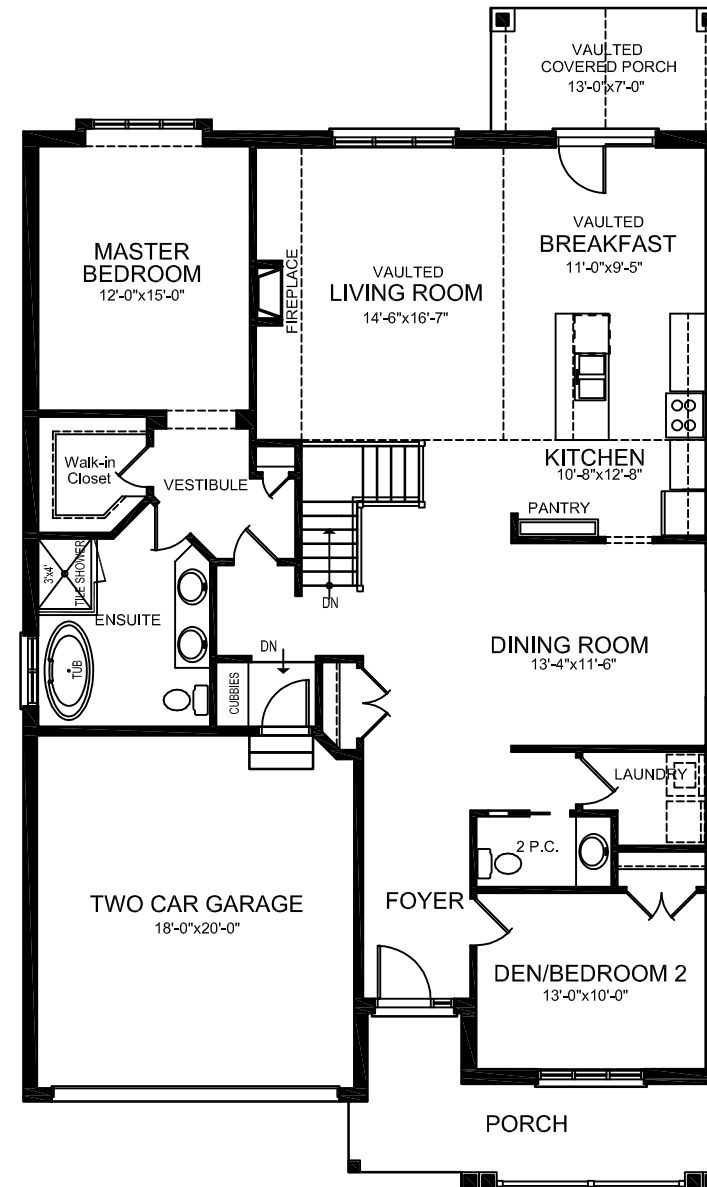
MAIN FLOOR PLAN-1741 sq.ft.
