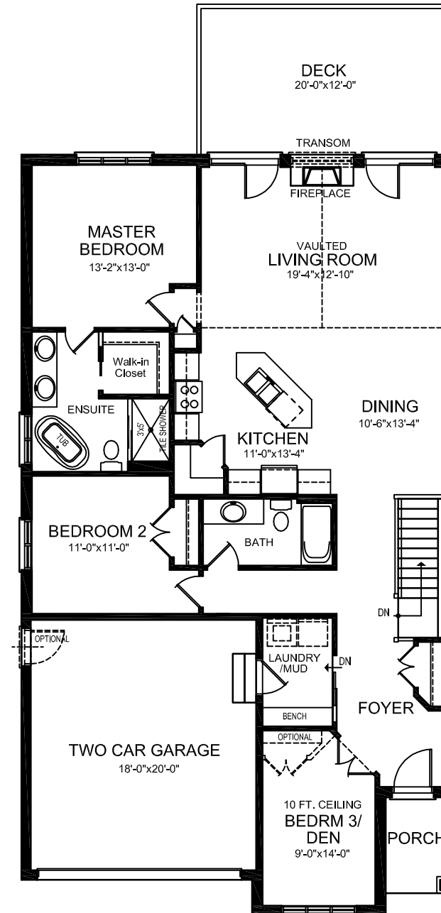
MAIN FLOOR PLAN - 1605 SQ.FT.
