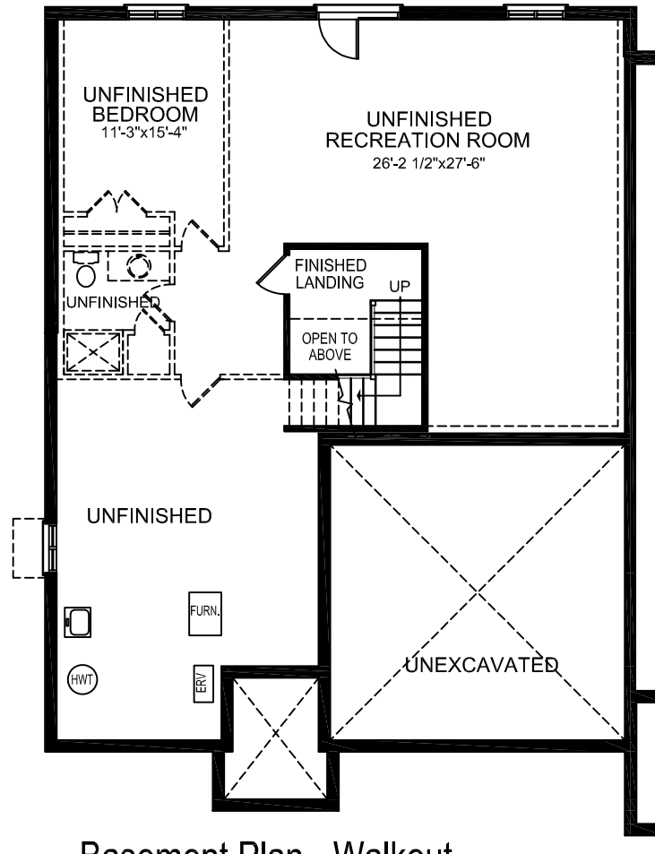
Basement Plan - Walkout
