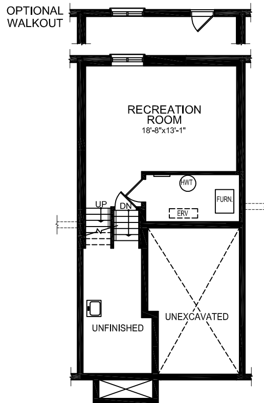
Basement Plan
