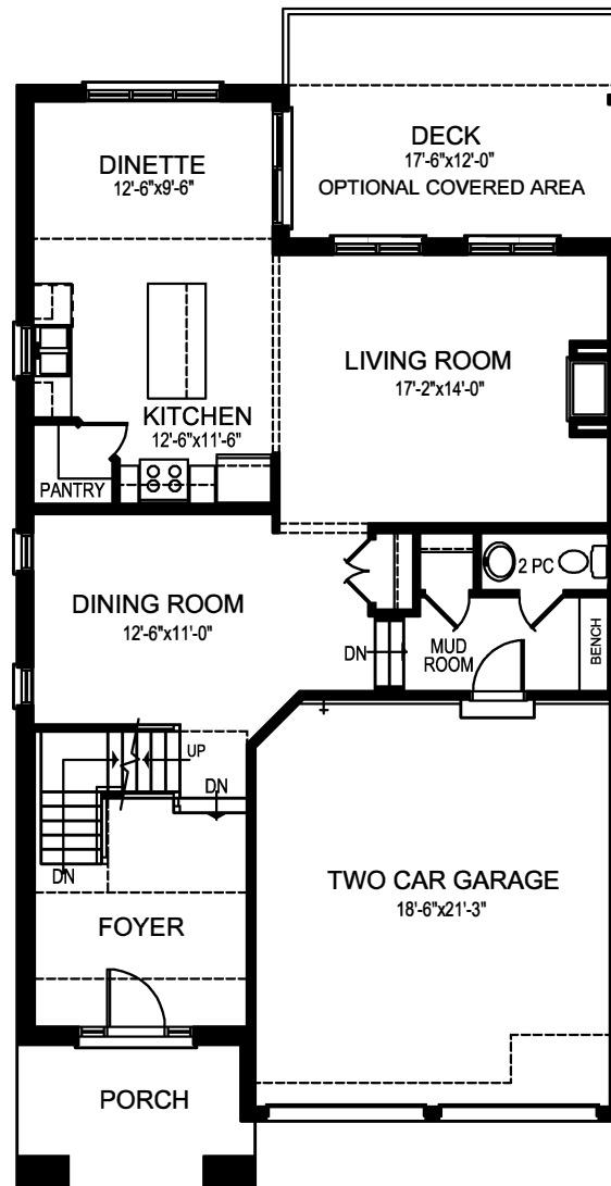
MAIN FLOOR PLAN - 1100 sq.ft.
