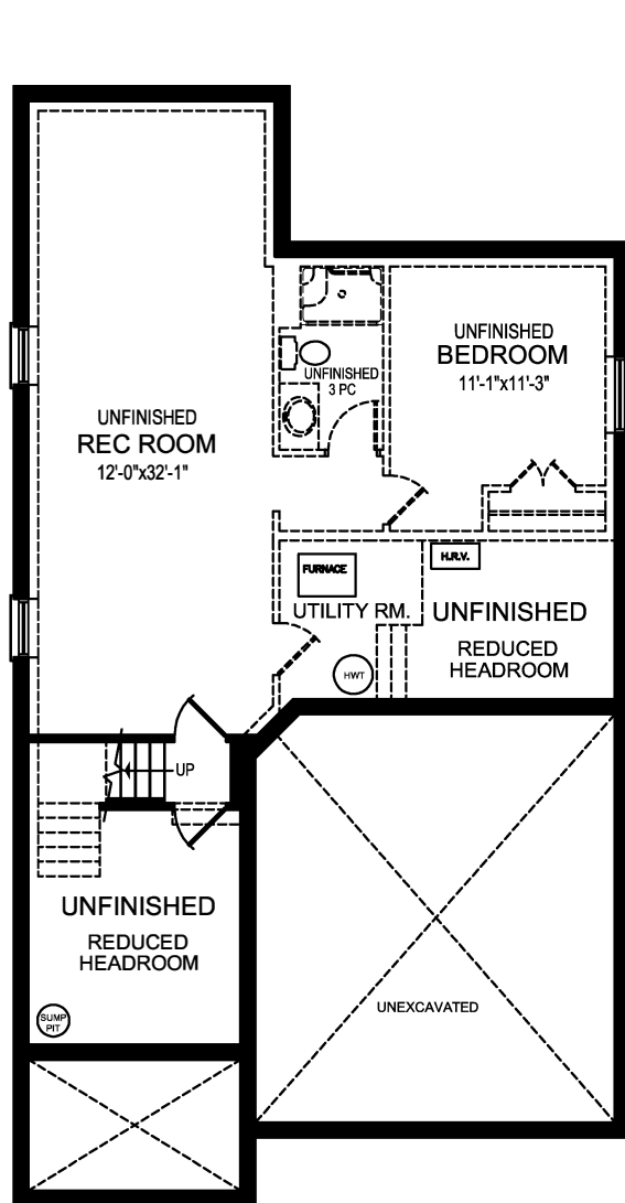
UNFINISHED BASEMENT PLAN OPTIONAL FINISHED AREA 780 SQ.FT.
