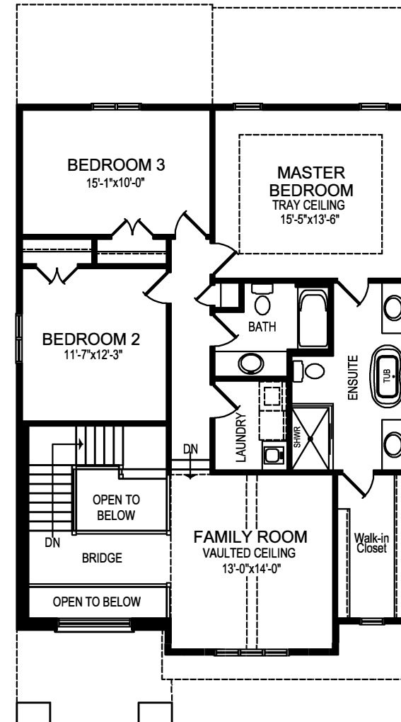
SECOND FLOOR PLAN - 1294 sq.ft. PLUS 60 SQ.FT. SPACE OPEN TO BELOW
