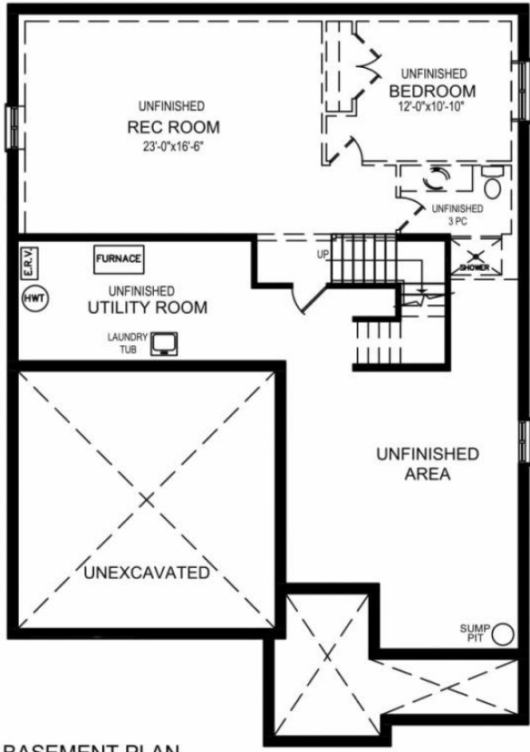
BASEMENT PLAN FUTURE FINISHED AREA = 853 SQ.FT.
