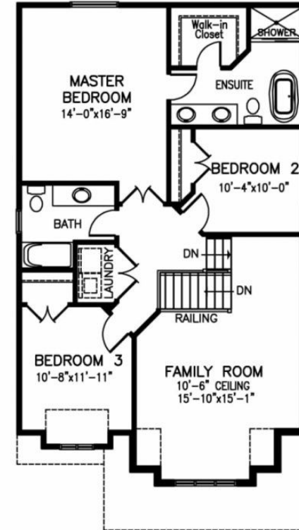
SECOND FLOOR PLAN - 1229 SQ.FT.
